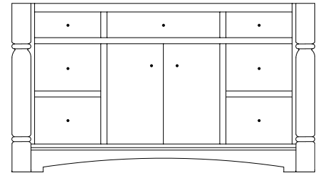
DSL-751 61¾"w 34½"h 24½"d w/7 drawers, 2 doors
