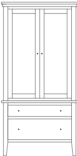
CS-1662 Armoire 40 \frac{1}{2} "w 78"h 21 \frac{1}{2} "d w/2 drawers, (top drawer w/divider) w/2 doors, 2 adj. shelves & closet rod
