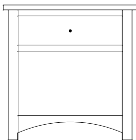
CM-1543 Night Stand 27½"w 27¾"h 17½"d w/1 drawer
