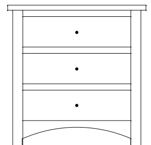
CM-1545 Night Stand 27½"w 27¾"h 17½"d w/3 drawers
