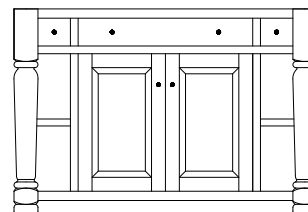
IS-96 49"w 34½"h 24½"d w/3 drawers, 2 doors w/1 adjustable shelf, 2 open shelves
