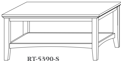
RT-5390-S 41½"w x 19½"h x 23½"d Coffee Table w/1 Open Shelf
