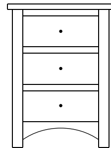
MH-2142 Night Stand 20¾"w 27¾"h 17½"d w/3 drawers
